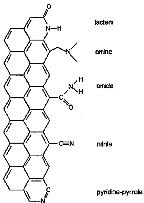
Figure 1. Nitrogen functional groups on a hypothetical carbon surface, introduced from treatment of the carbon with ammonia (adapted from Jansen and vanBekum, 1994).
