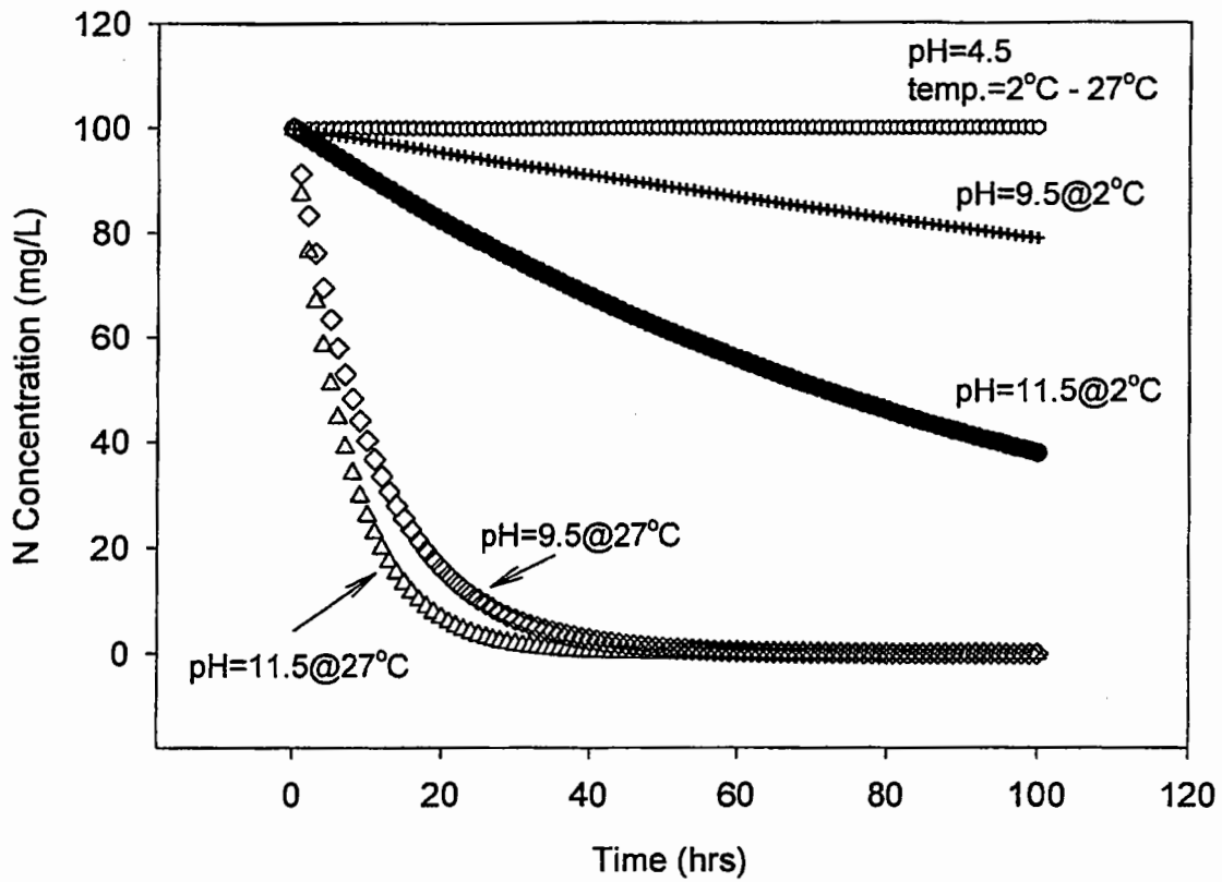
Figure 6. The effect of temperature on the rate of ammonia loss from water at different pH levels (calculated from Weiler, 1979).
