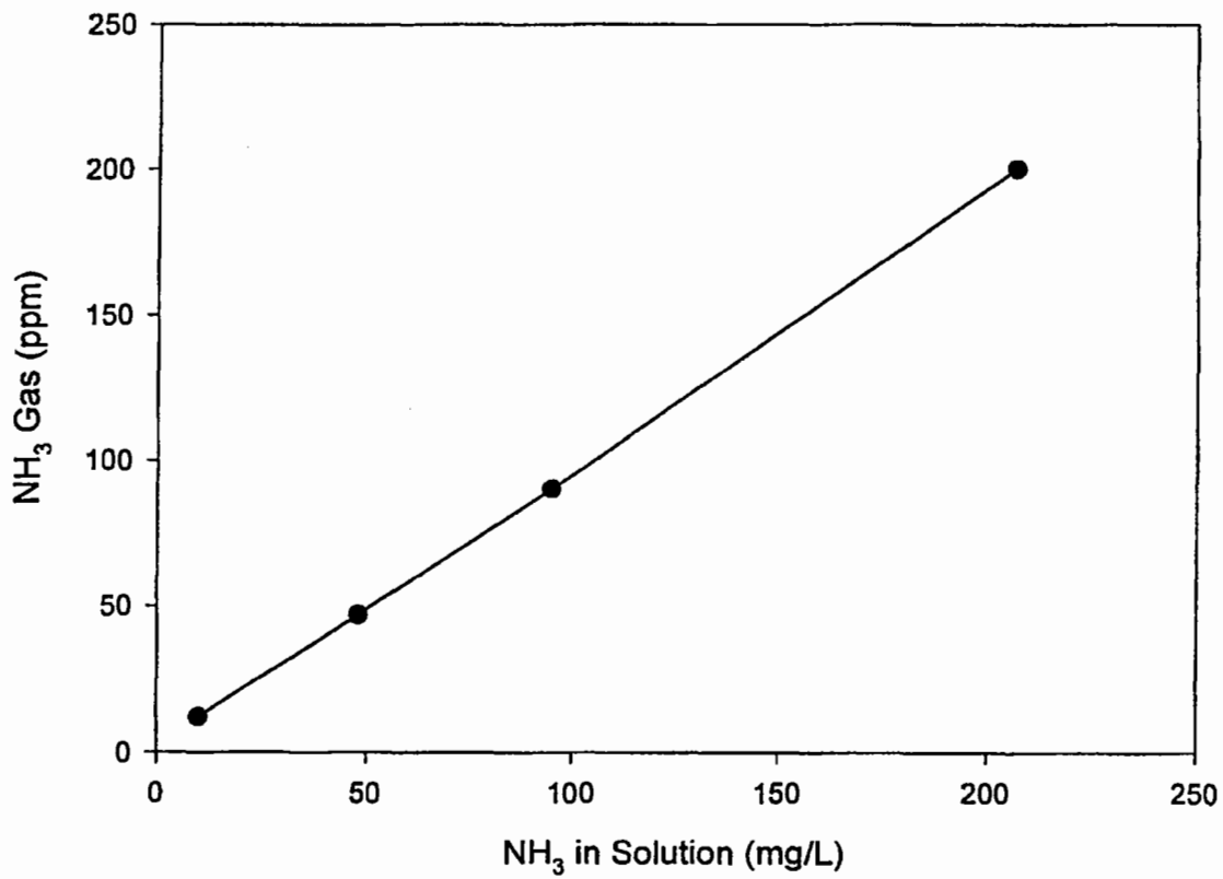
Figure 7. Calibration curve for the GasTec 3La ammonia detection tube.
