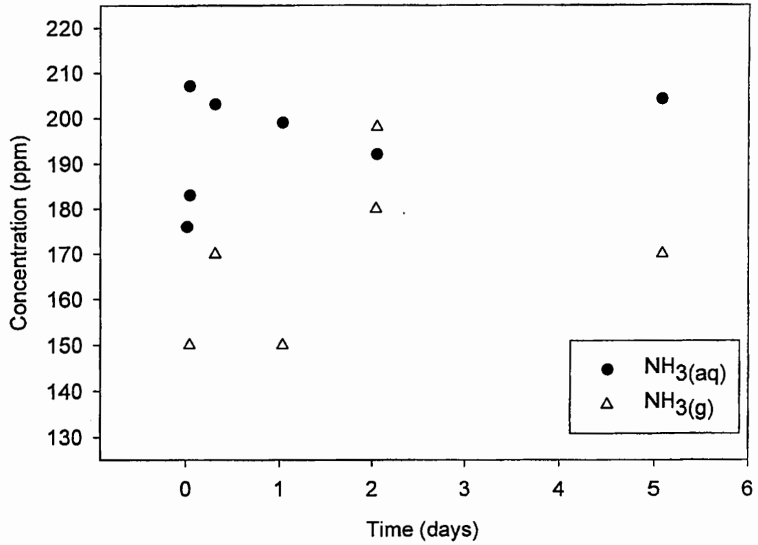
Figure 8. Ammonia release from fly ash "W" in distilled water under closed conditions.
